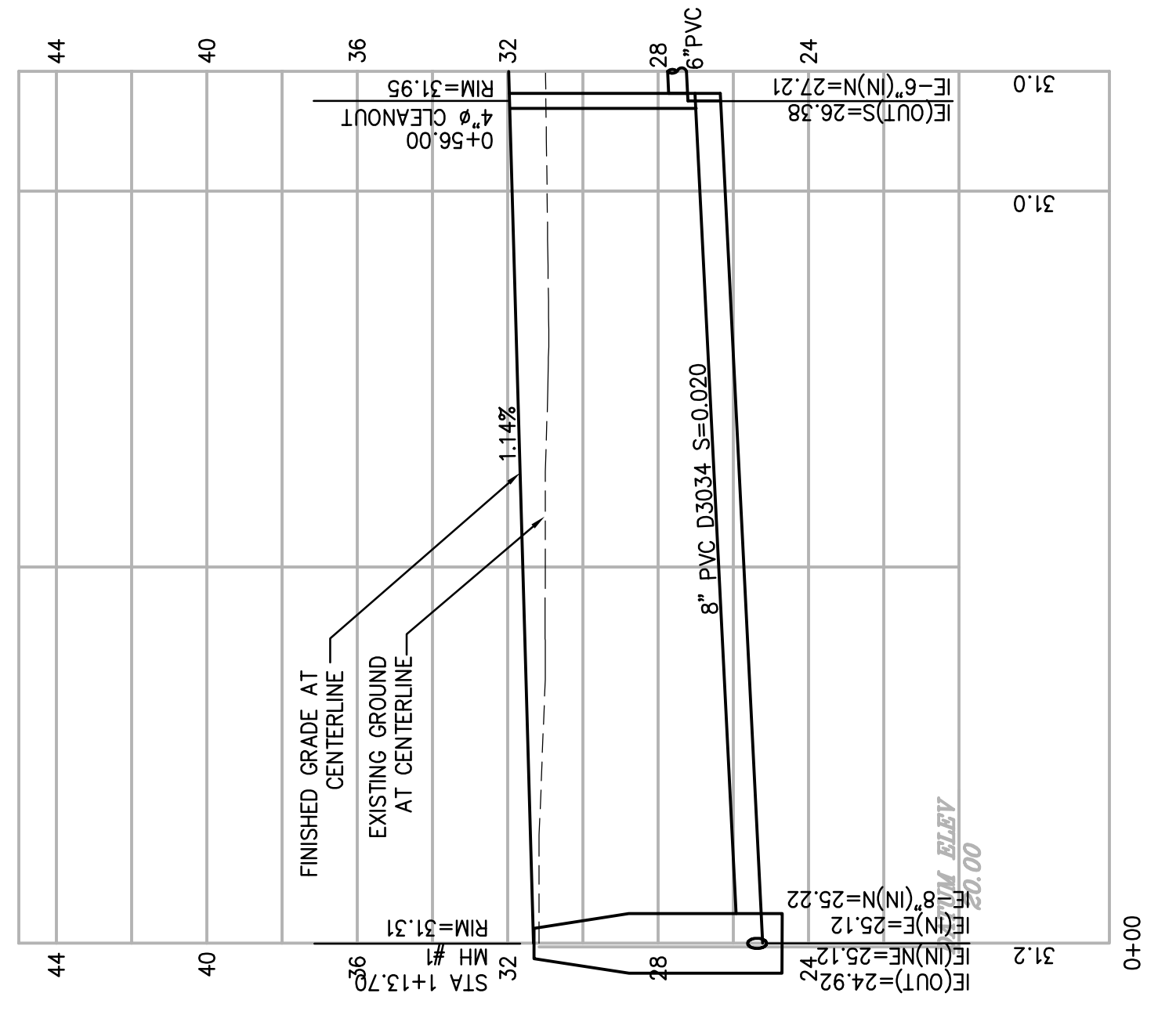
LINE-B SANITARY SEWER PROFILE SCALE: H: 1"=10' V: 1"=4'
