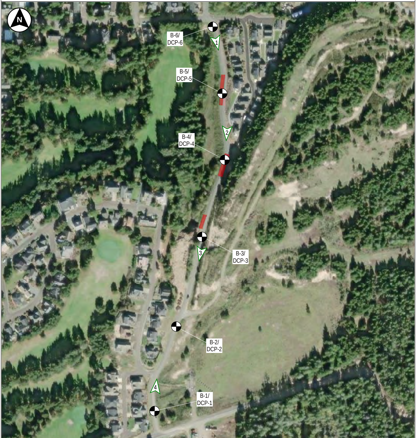
FIGURE 2 Site Plan
